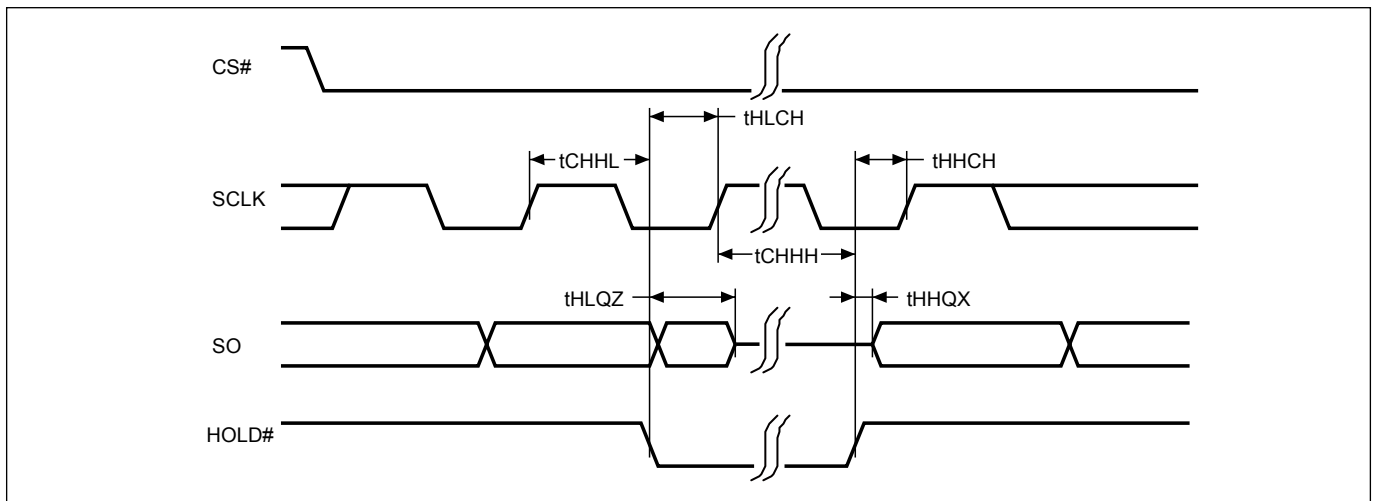
Figure 4. Hold Timing
