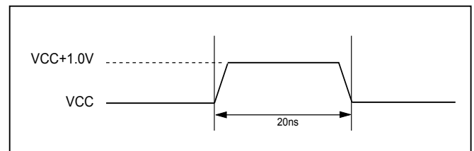
Figure 48. Maximum Positive Overshoot Waveform
