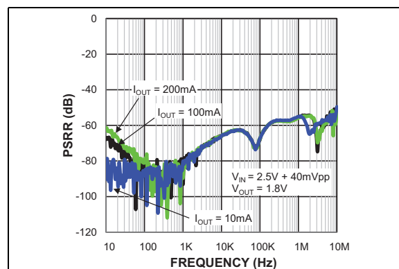
FIGURE 2-5: PSRR C_{OUT} = 2.2 \mu F .
