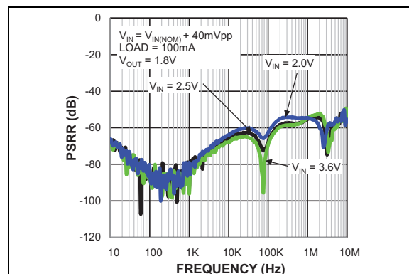
FIGURE 2-6: PSRR C_{OUT} = 2.2 \mu F .
