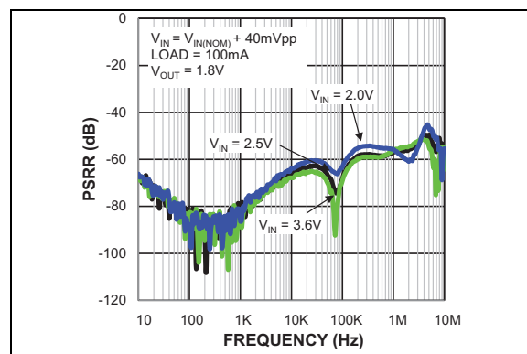
FIGURE 2-4: PSRR C_{OUT} = 1 \mu F .
