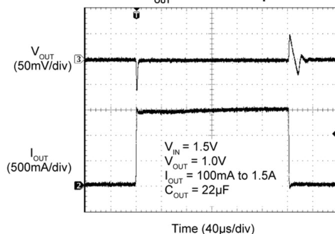
Transient Response V_{OUT} = 1.0V with 22µF
