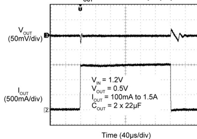
Transient Response V_{OUT} = 0.5V with 22µF (x2)
