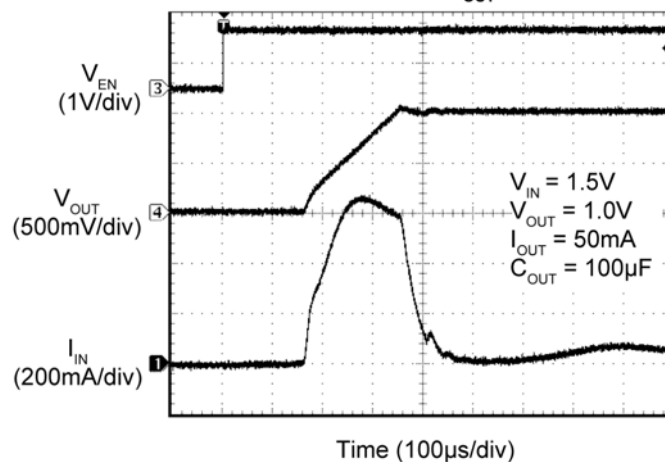
Inrush Current, C_{OUT} = 100\mu F
