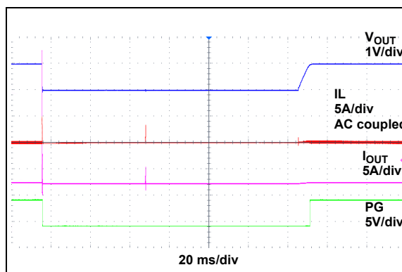
FIGURE 2-32: Hiccup Mode Short Circuit Current Limit Response.
