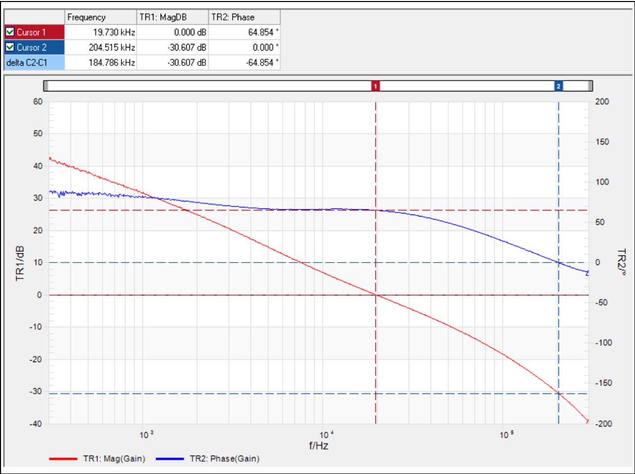
FIGURE 2-40: Voltage Loop Gain Bode Plot, V_{OUT} = 1.8V , f_s = 570\text{ kHz} , L = 1.2\text{ }\mu H , C_{OUT} = 266\text{ }\mu F , R_{C1} = 2.55k\Omega , C_{C1} = 10nF , C_{C2} = 47pF (see Section 7.7, Compensation Design ).
