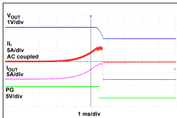
FIGURE 2-31: Output Current Limit Threshold.
