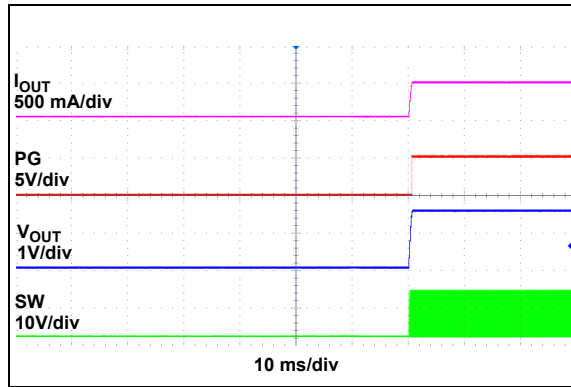
FIGURE 2-34: Recovery from Thermal Shutdown.
