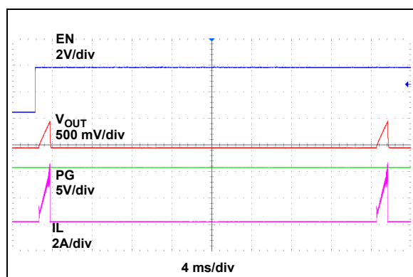
FIGURE 2-30: Enable into Short Circuit.
