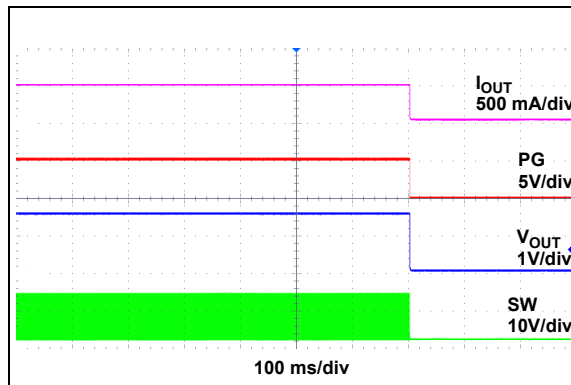
FIGURE 2-33: Thermal Shutdown Response.
