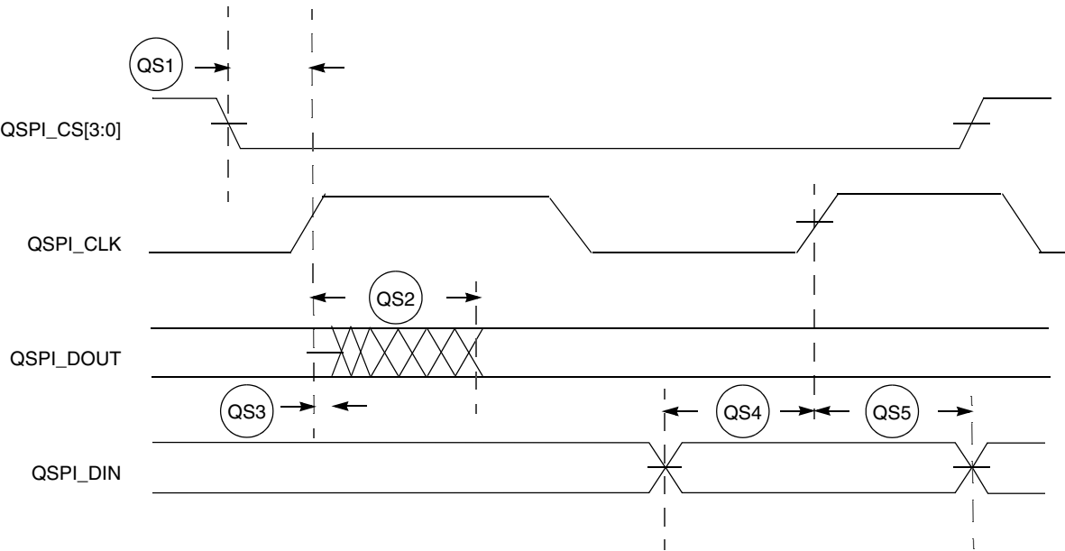
Figure 13. QSPI Timing
