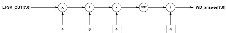
Figure 15. Watchdog answer calculation
