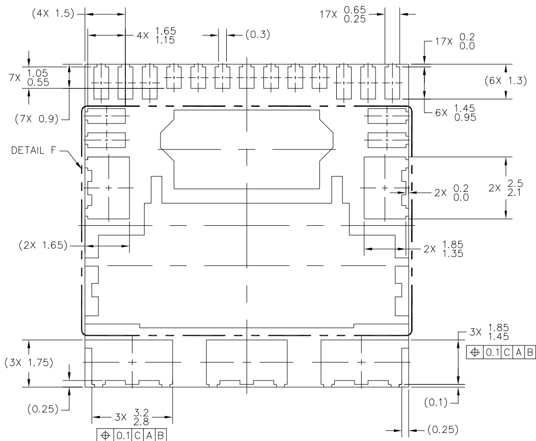
DETAIL E
