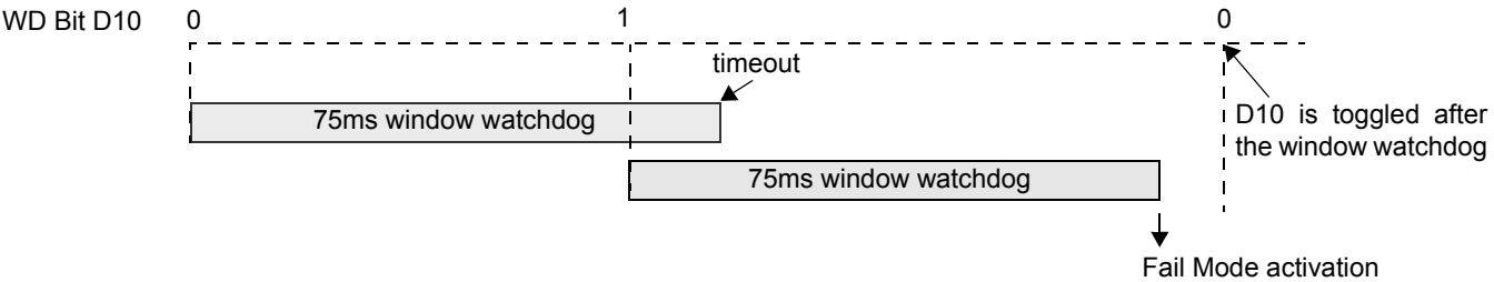
Figure 18. Watchdog window
