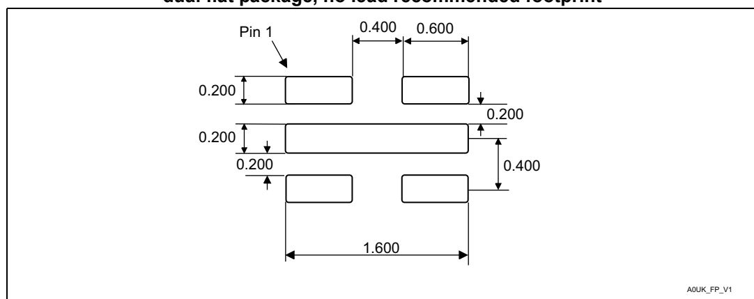
Figure 14. UDFPN5 - 5-lead, 1.7 × 1.4 mm, 0.55 mm thickness, ultra thin fine pitch dual flat package, no lead recommended footprint
