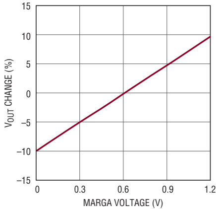
Output Voltage Change vs MARGA Voltage, 1V_{OUT}
