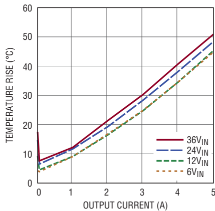
Temperature Rise vs Output Current, 1.2V_{OUT}
