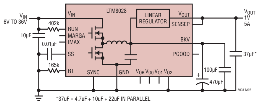
1V at 5A Regulator
