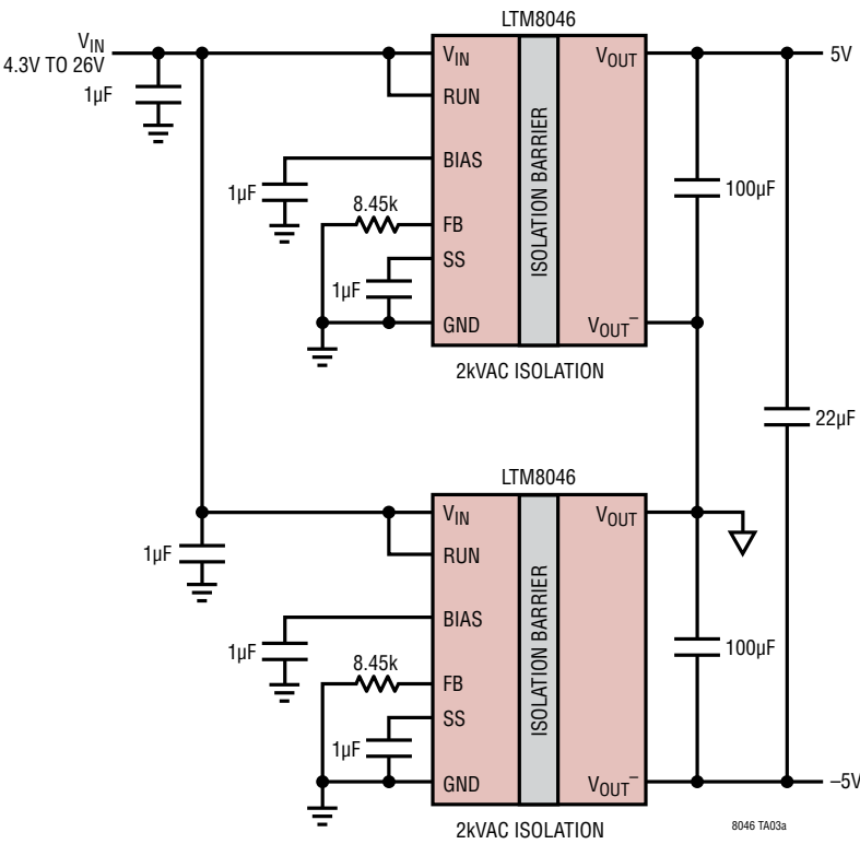
Use Two LTM8046 Flyback Converters to Generate ±5V
