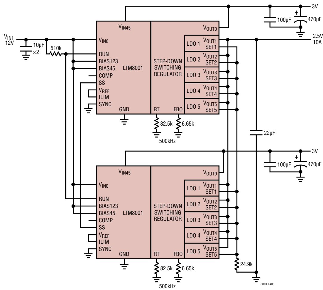
Use Two LTM8001s to Implement a 2.5V OUT 10A DC/DC μModule Converter
