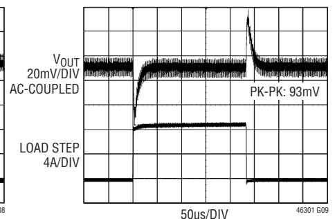
Dual Phase Single Output 25% (9A) Transient Response at 1.8V Output
