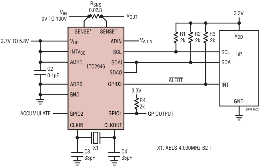
Rail-to-Rail Power, Charge and Energy Monitor
