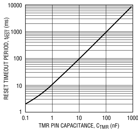
External Timeout Period vs Capacitance
