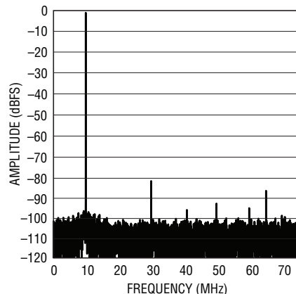
LTC2262-14: 8k Point FFT, f_{IN} = 140\text{MHz} -1dBFS, 150Mps
