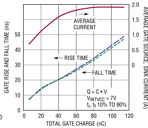
GATE Rise and Fall Time vs Charge
