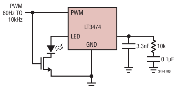
Figure 7. Dimming Using PWM Signal
