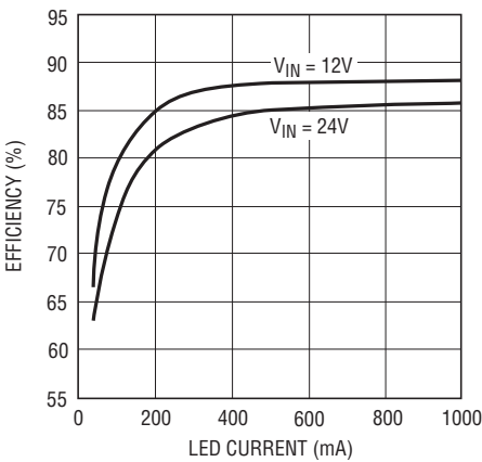
Efficiency, Two LED Output
