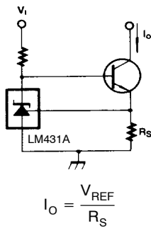
Figure 16. Constant-Current Sink
