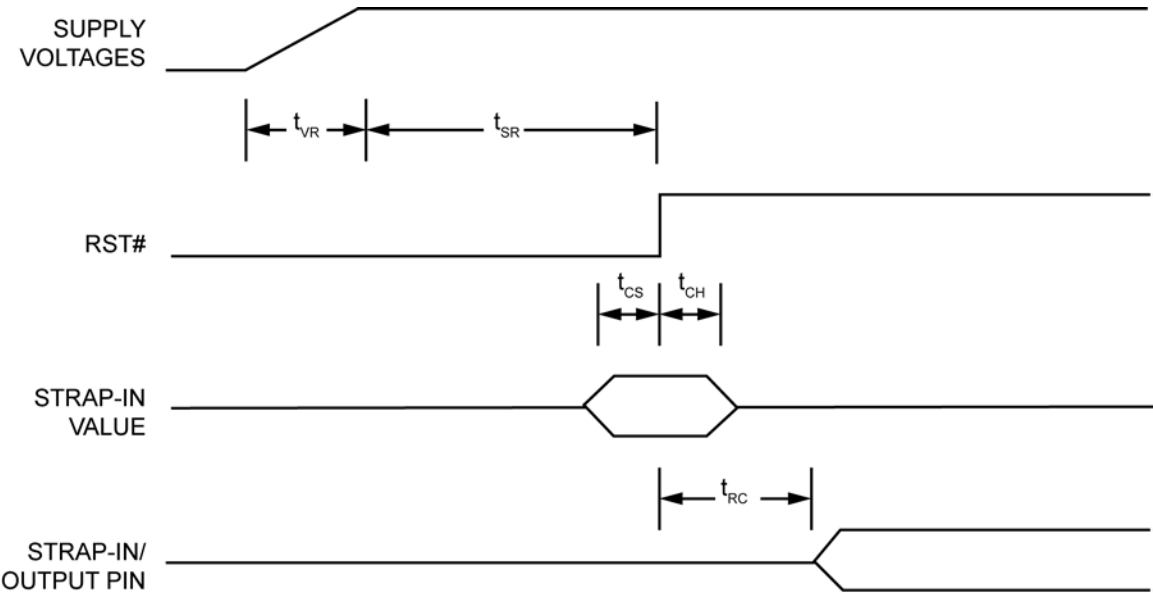
Figure 17. Power-Up/Reset Timing
