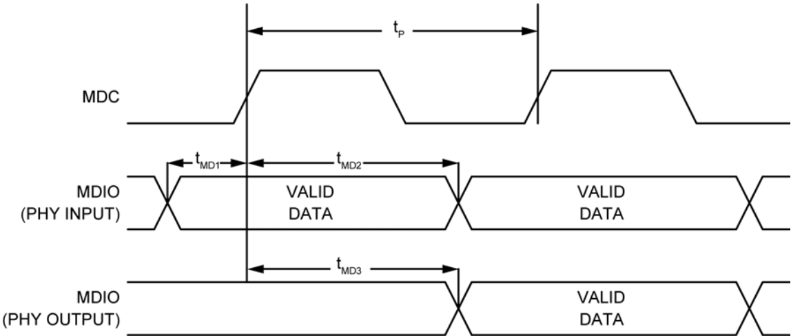
Figure 16. MDC/MDIO Timing
