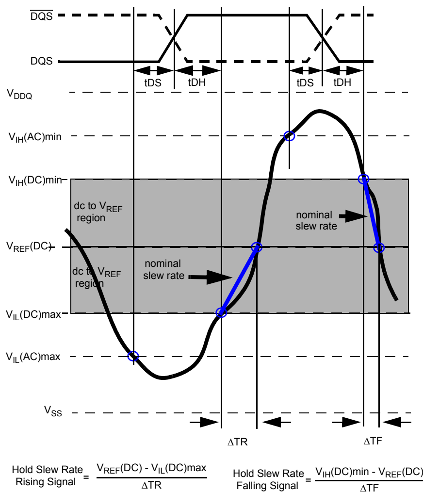
Figure 11. Illustration of nominal slew rate for tDH (differential DQS, DQS)
