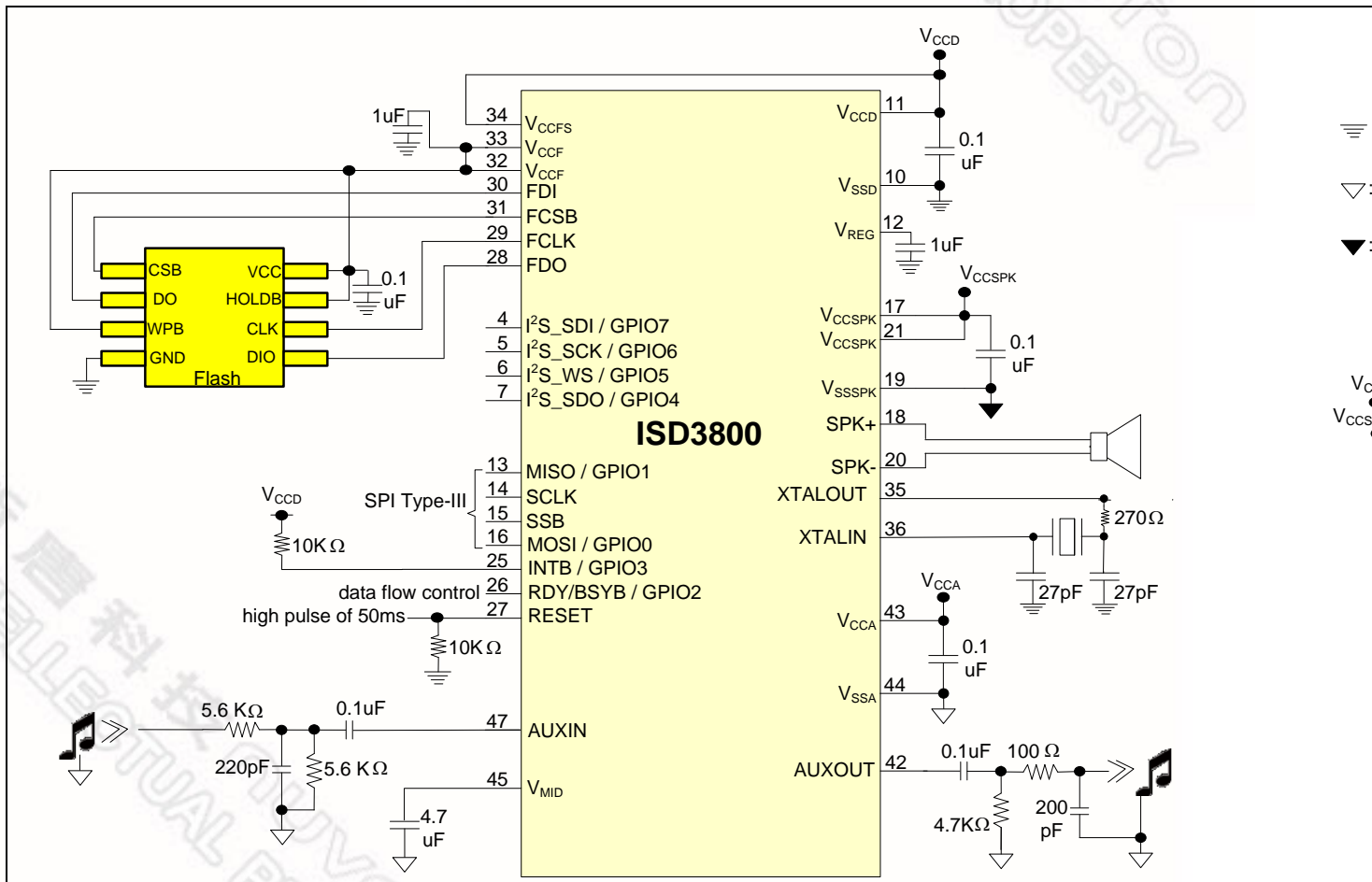
Figure 7-1 ISD3800 Application Diagram – V_{CCF} is regulated internally from V_{CCFS}
