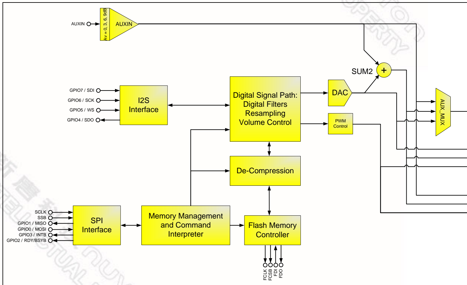
Figure 3-1 ISD3800 Block Diagram
