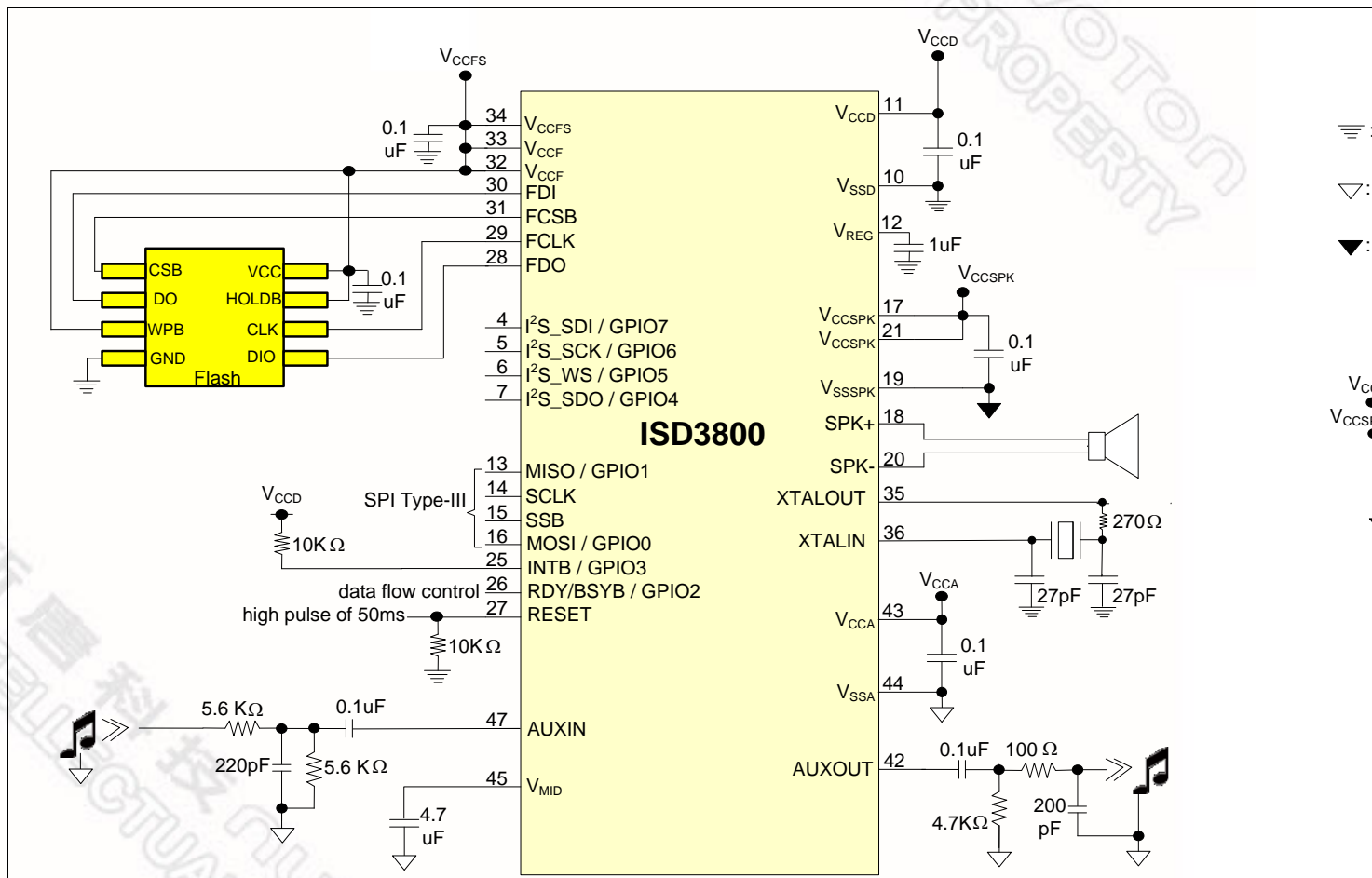
Figure 7-2 ISD3800 Application Diagram – V_{CCF} is tied to V_{CCFS}
