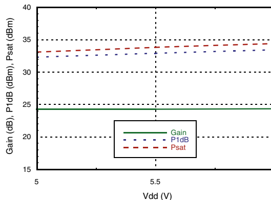
Gain & Power vs. Supply Voltage @ 29.5 GHz
