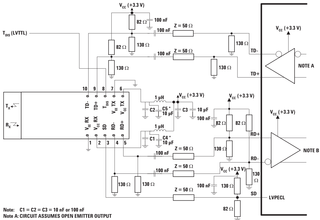
Figure 6b. Recommended ac Coupled Interface Circuit
