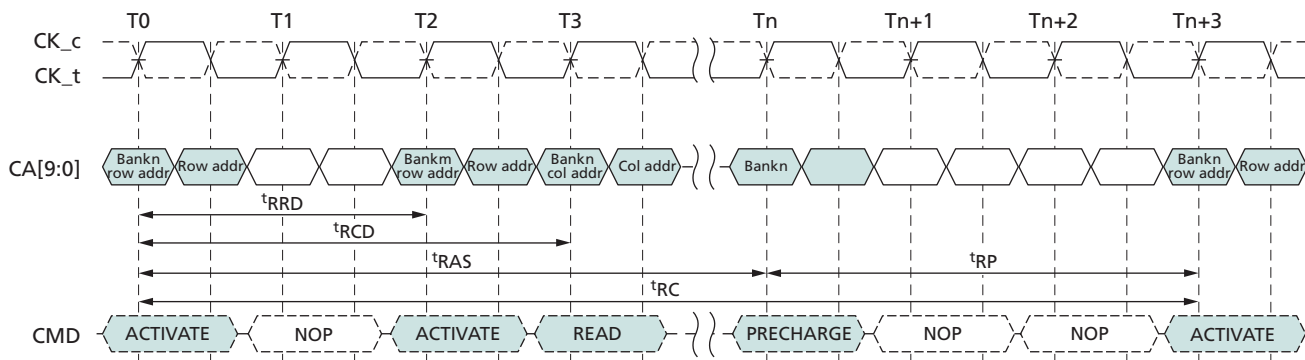
Figure 15: ACTIVATE Command
