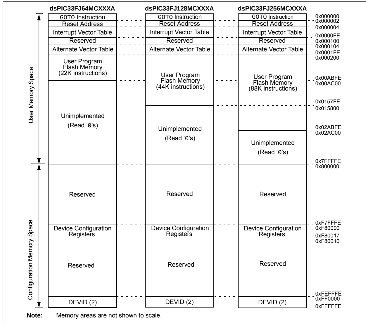
FIGURE 4-1: PROGRAM MEMORY MAP FOR dsPIC33FJXXMXX06A/X08A/X10A DEVICES
