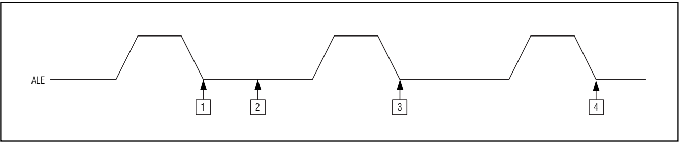
Figure 8. ALE Waveform
