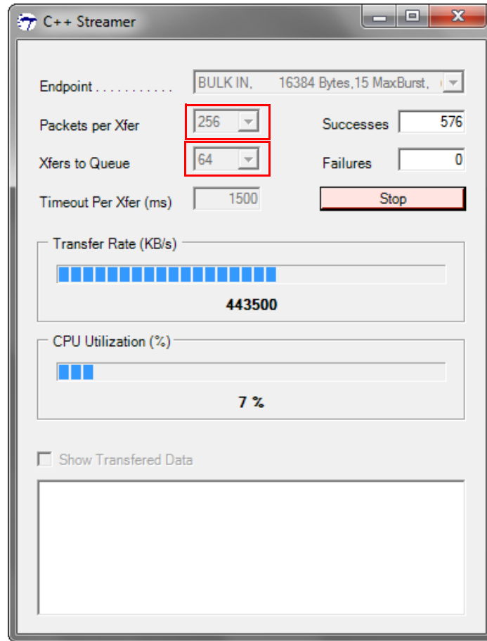
Figure 3-11. Streamer.exe
