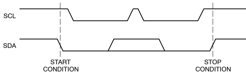
Figure 6. START/STOP Condition
