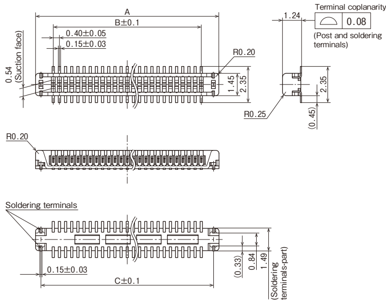
External dimensions
