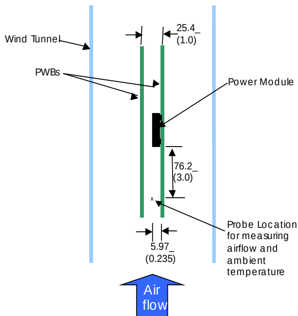
Figure 34. Thermal Test Set-up.
