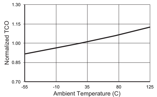
Normalized TCO vs Ambient Temperature
