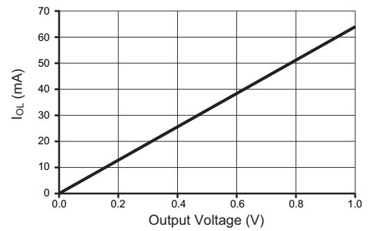
Output Sink Current vs Output Voltage
