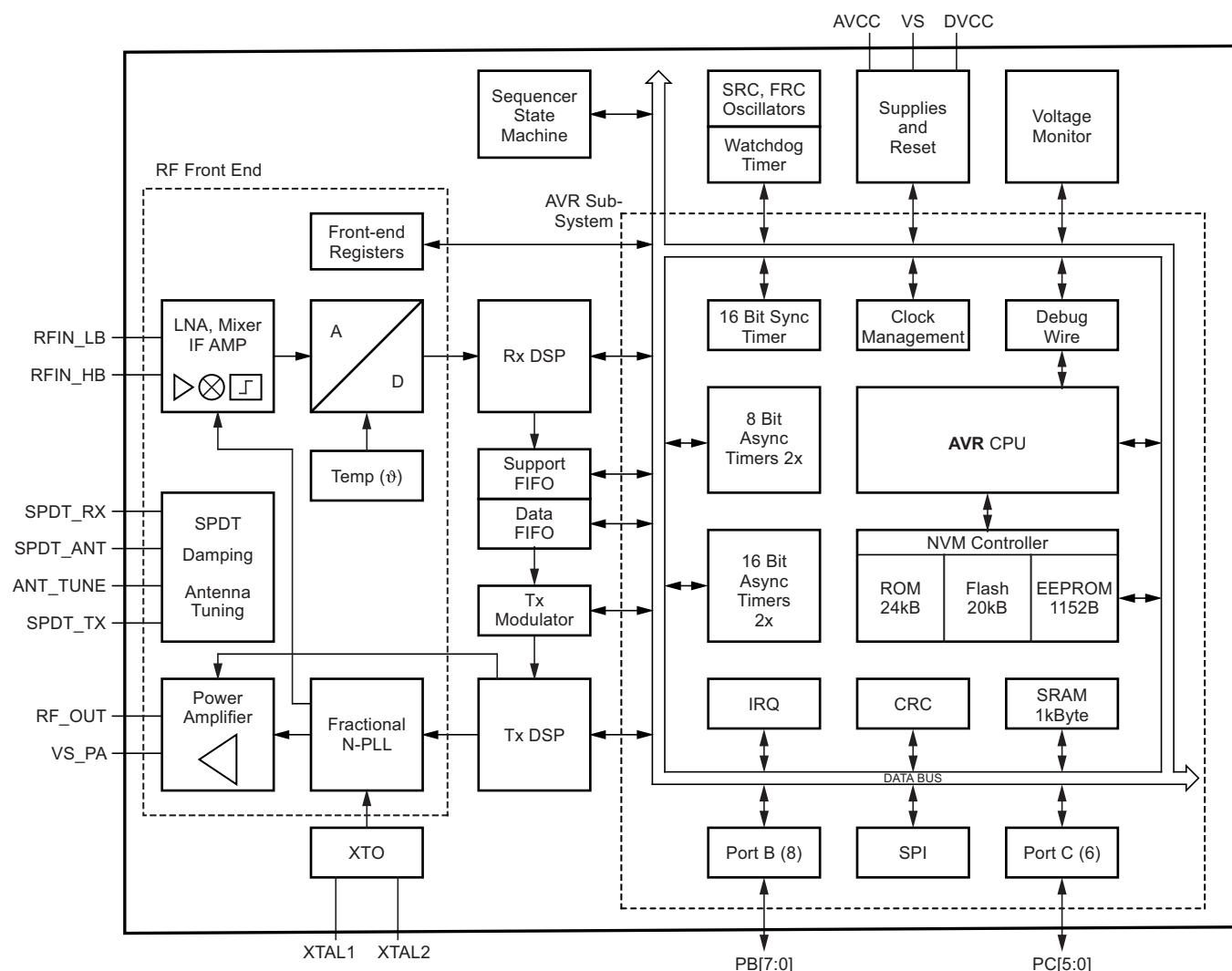
Figure 3-1. Block Diagram
