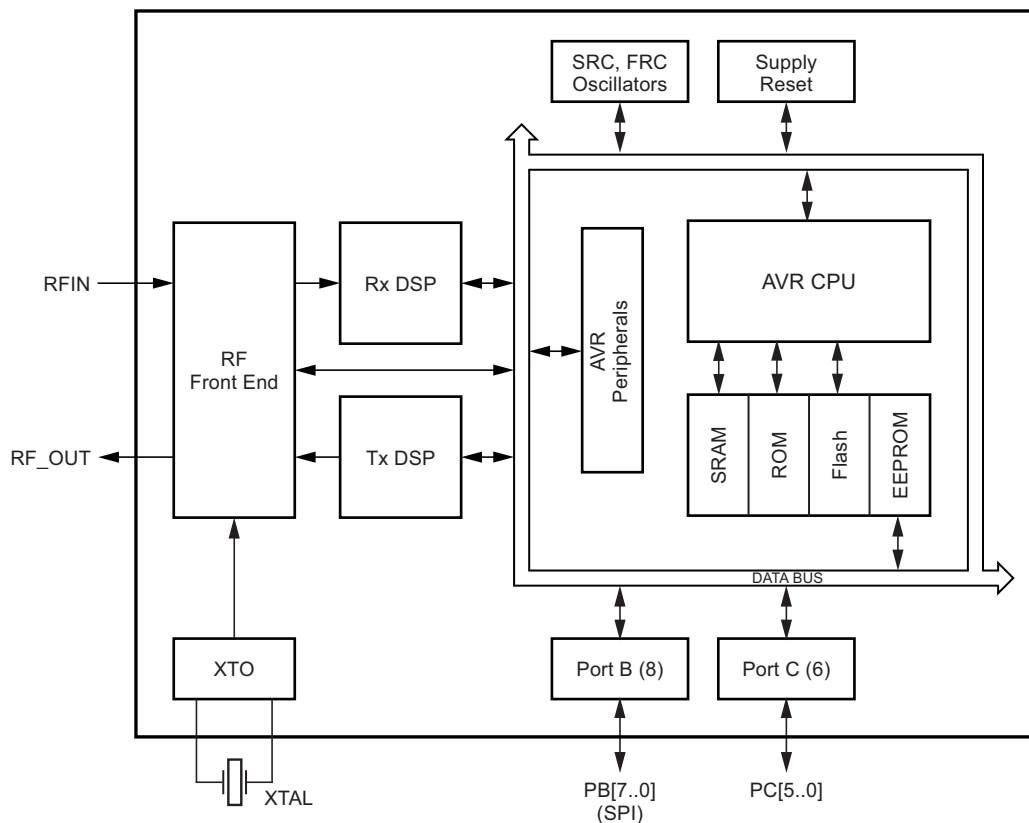
Figure 1-1. Circuit Overview
