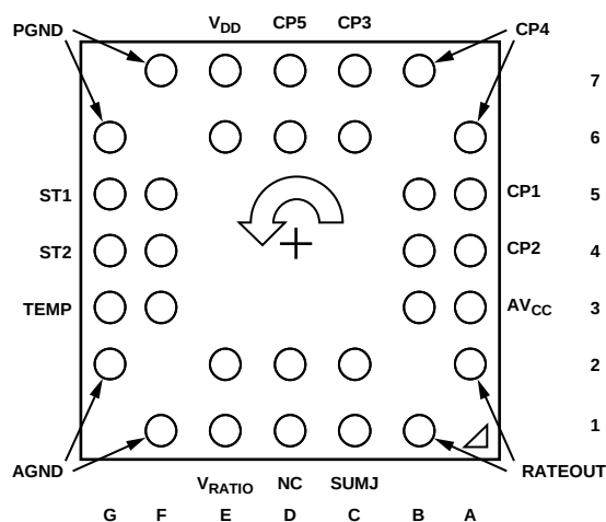
Figure 3. Pin Configuration
