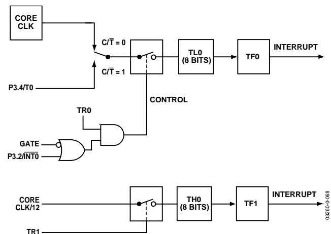
Figure 69. Timer/Counter 0, Mode 3
