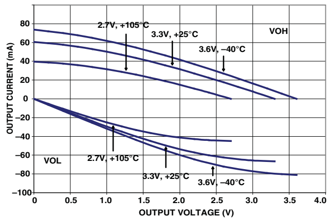
Figure 67. Drive Current C (High V_{DDEXT} )
