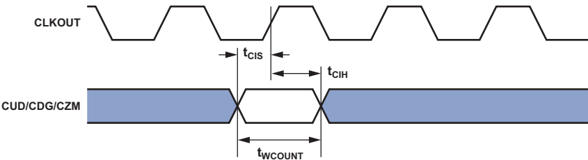
Figure 43. Up/Down Counter/Rotary Encoder Timing
