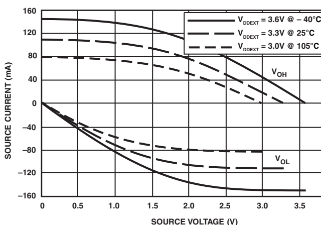
Figure 52. Driver Type D Current ( 3.3V_{DDEXT}/V_{DDMEM} )
