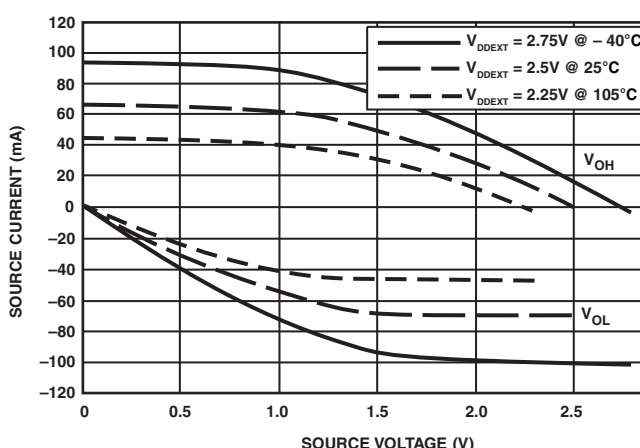
Figure 53. Driver Type D Current ( 2.5V_{DDEXT}/V_{DDMEM} )
