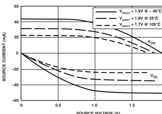
Figure 54. Driver Type D Current ( 1.8V_{DDEXT}/V_{DDMEM} )
