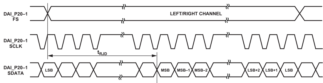
Figure 31. Right-Justified Mode
