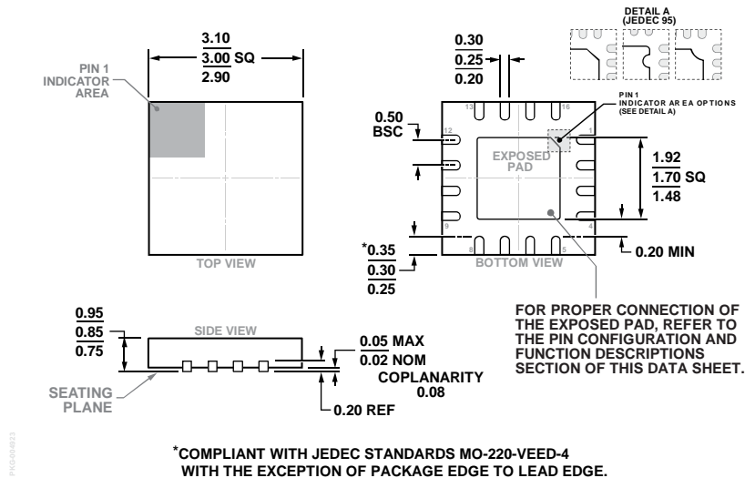
Figure 25. 16-Lead Lead Frame Chip Scale Package [LFCSP] 3 mm × 3 mm Body and 0.85 mm Package Height (CP-16-38) Dimensions shown in millimeters
