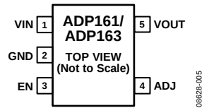
Figure 5. 5-Lead TSOT, Adjustable Output Pin Configuration, ADP161/ADP163
