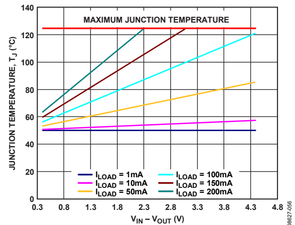
Figure 55. LFCSP 100 mm² of PCB Copper, T_A = 50^\circ\text{C}
