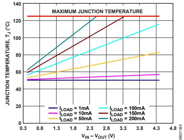
Figure 54. LFCSP 500 mm² of PCB Copper, T_A = 50^\circ\text{C}
