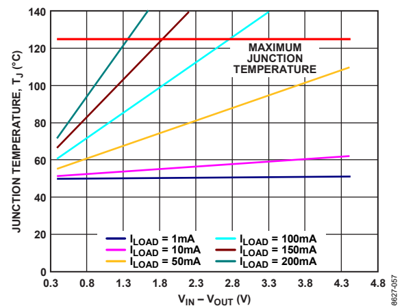
Figure 56. LFCSP 50 mm² of PCB Copper, T_A = 50^\circ\text{C}
