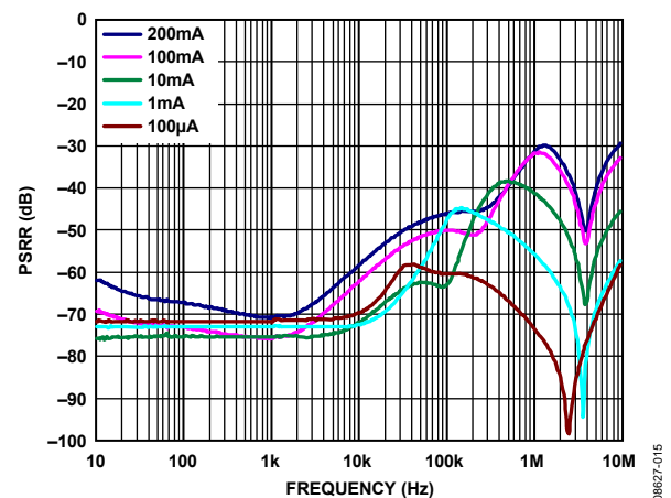
Figure 17. PSRR vs. Frequency, V_{OUT} = 1.2 V , V_{IN} = 2.2 V
