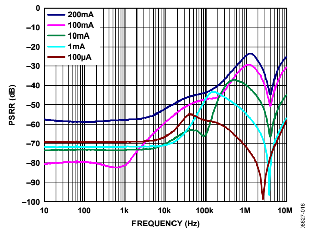
Figure 18. PSRR vs. Frequency, V_{OUT} = 2.8 V , V_{IN} = 3.3 V
