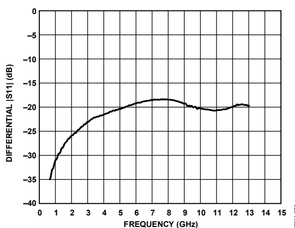
Figure 10. Differential |S11|
