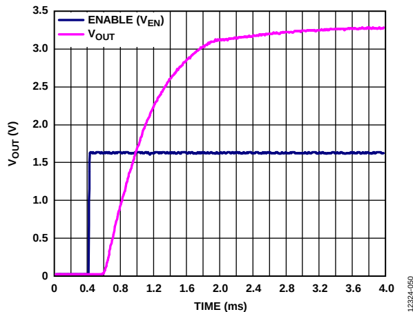
Figure 50. Typical V OUT Response to EN Pin Operation (V EN ), V OUT = 3.3 V, V IN = 5 V, C BYP = 1 μF
