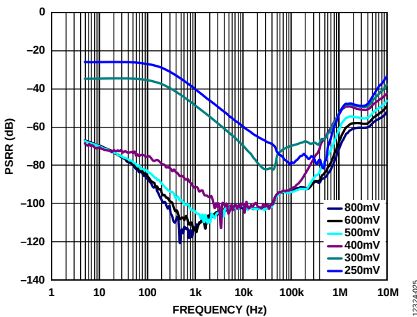
Figure 25. Power Supply Rejection Ratio (PSRR) vs. Frequency at Various Headroom Voltages, V_{OUT} = 1.8\text{ V} , 400 mA Load
