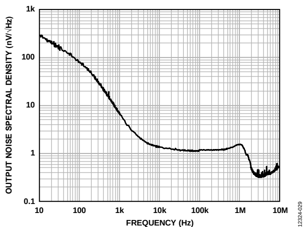
Figure 30. Output Noise Spectral Density, 10 Hz to 10 MHz, I_{LOAD} = 100\text{ mA}
