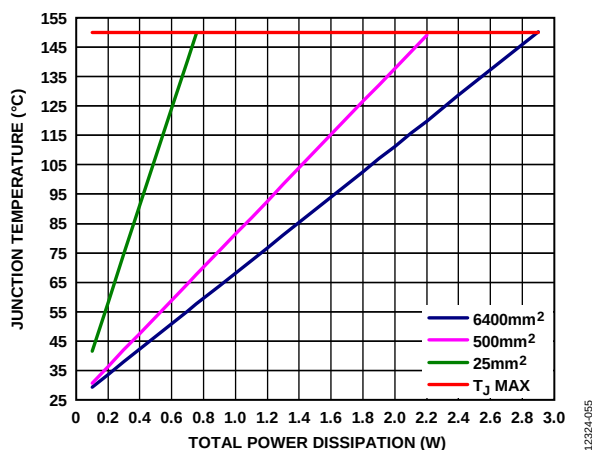
Figure 55. Junction Temperature vs. Total Power Dissipation for the 8-Lead LFCSP, T_A = 25^\circ\text{C}
