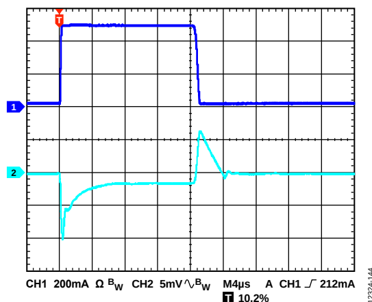
Figure 44. Output Transient Response, V_{OUT} = 3.3\text{ V} , C_{OUT} = 10\text{ }\mu\text{F} , CH1 = Load Current, CH2 = V_{OUT}
