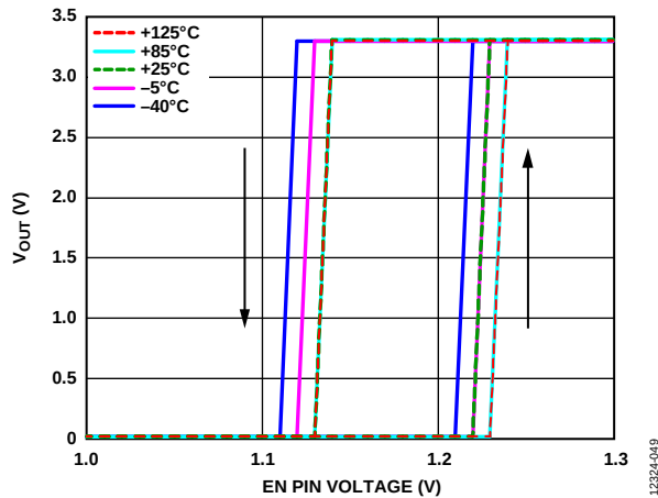
Figure 49. Typical V OUT Response to EN Pin Operation
