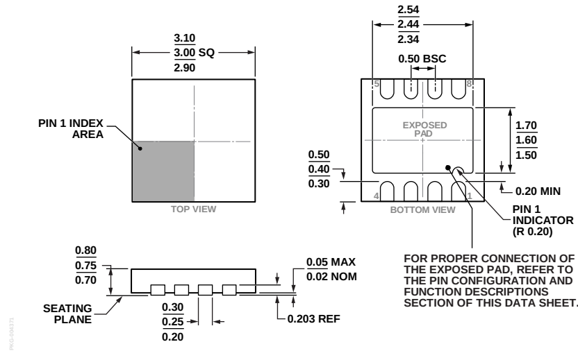
Figure 65. 8-Lead Lead Frame Chip Scale Package [LFCSP_WD] 3 mm x 3 mm Body, Very Very Thin, Dual Lead (CP-8-21) Dimensions shown in millimeters
