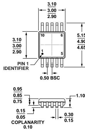
Figure 25. 10-Lead Mini Small Outline Package [MSOP] (RM-10)
