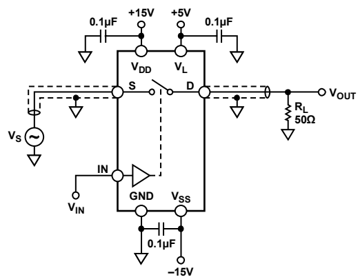
Figure 22. Off Isolation
