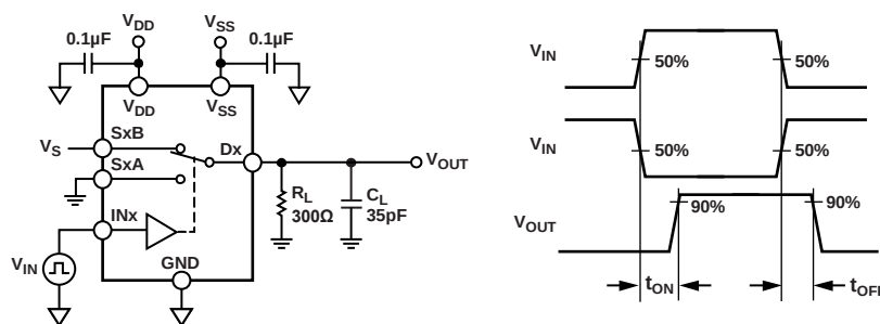
Figure 30. Switching Times
