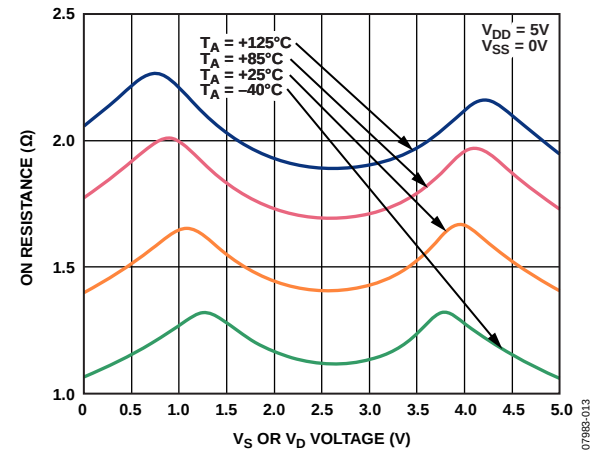
Figure 9. On Resistance as a Function of V_D ( V_S ) for Different Temperatures, 5 V Single Supply
