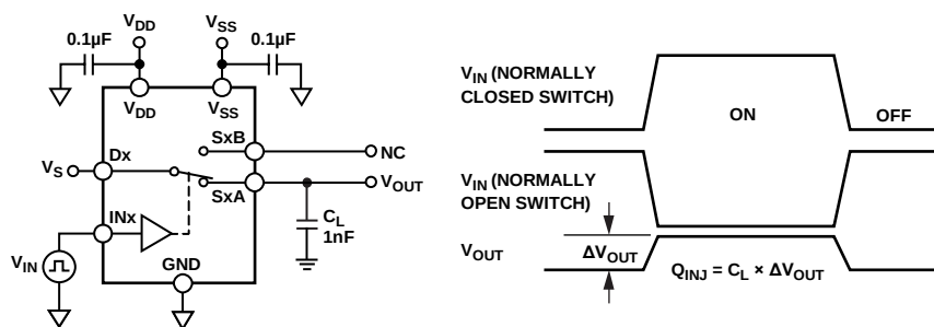
Figure 32. Charge Injection
