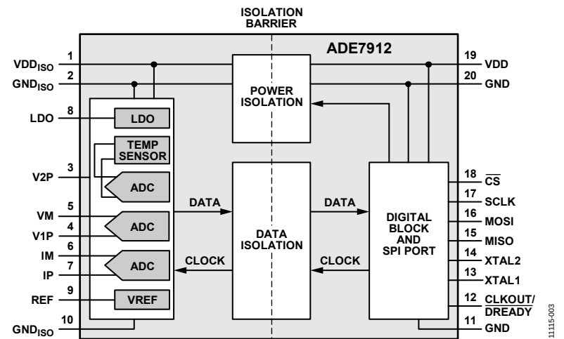
Figure 2. ADE7912 Functional Block Diagram
