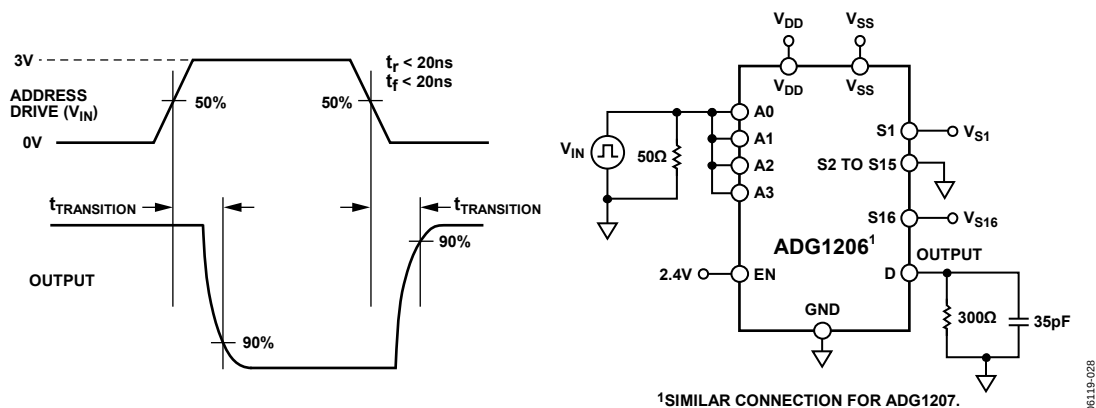
Figure 31. Address to Output Switching Times, t_{\text{TRANSITION}}
