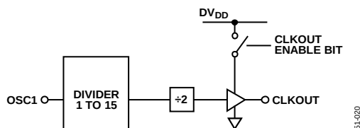
Figure 20. CLKOUT Stage
