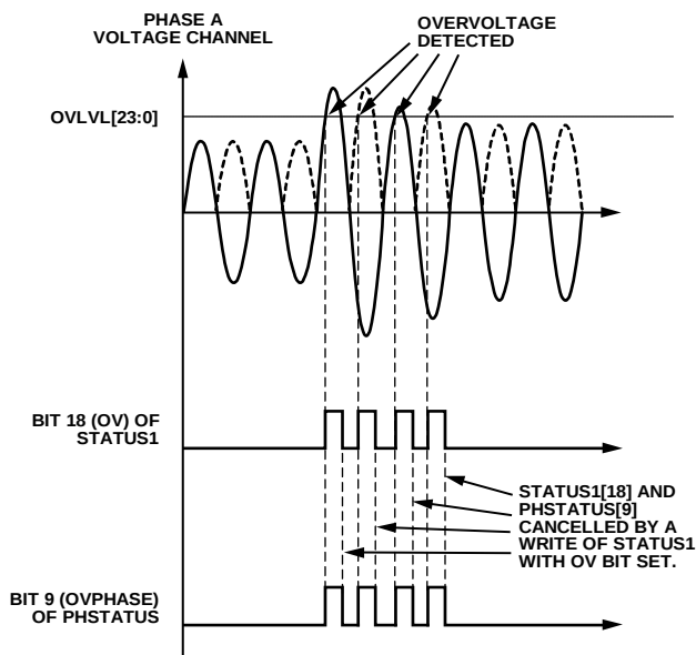
Figure 72. Overvoltage Detection
