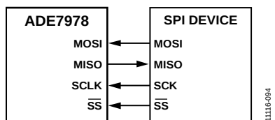
Figure 128. Connecting the ADE7978 SPI Interface to an SPI Device
