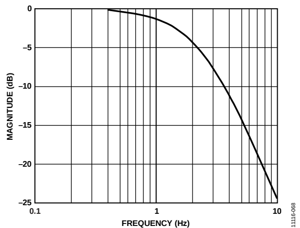
Figure 81. Frequency Response of the LPF Used to Filter Instantaneous Power in Each Phase: LPFSEL Bit of CONFIG Register Set to 0 (Default)
